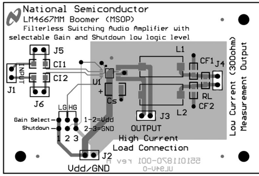
Composite View
